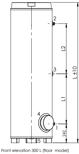
Front elevation 300 L (floor model)
